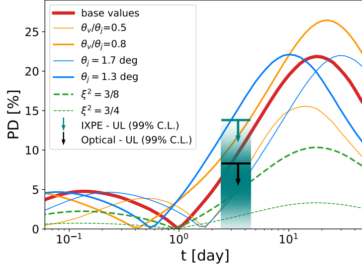
Figure 2. Polarization lightcurves using a set of base parameter values ( \theta_j = 1.5 deg, \theta_v = \frac{2}{3}\theta_j , p=2.96 , E_k = 10^{55} erg, A_* = 3 \times 10^{-1} cm ^{-1} , \xi = 0 ). We show the effect of changing the \theta_v/\theta_j ratio, the jet opening angle, \theta_j and the magnetic field ratio, \xi . The IXPE upper limits are shown in teal, while the black upper limit marks the upper limit of the contemporaneous optical observation. The shaded band shows a Gaussian modulation centered on the PD (darker shade) and width equal to the one sigma uncertainty on the PD (from the spectropolarimetric fit). We stress that we do not claim a measurement, which would require at least a 99% C.L. significance.
